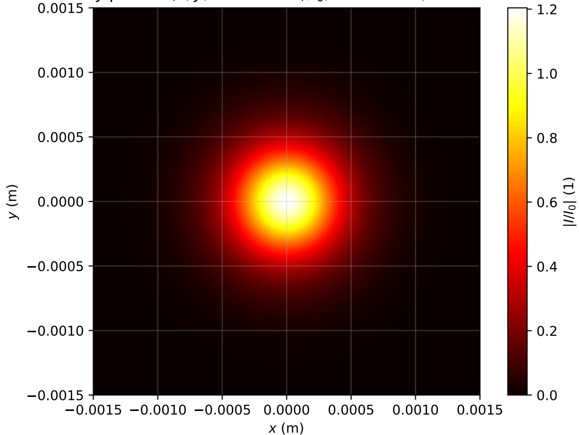
Intensity profile I(x, y, z = 1.035m)/I_0 , P_{in}=0.7P_{cr} , artificial time
